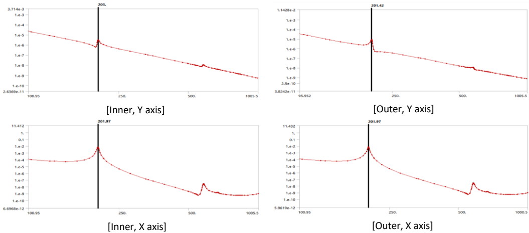
Figure 3. Vibration resonance graph of M12 nut
