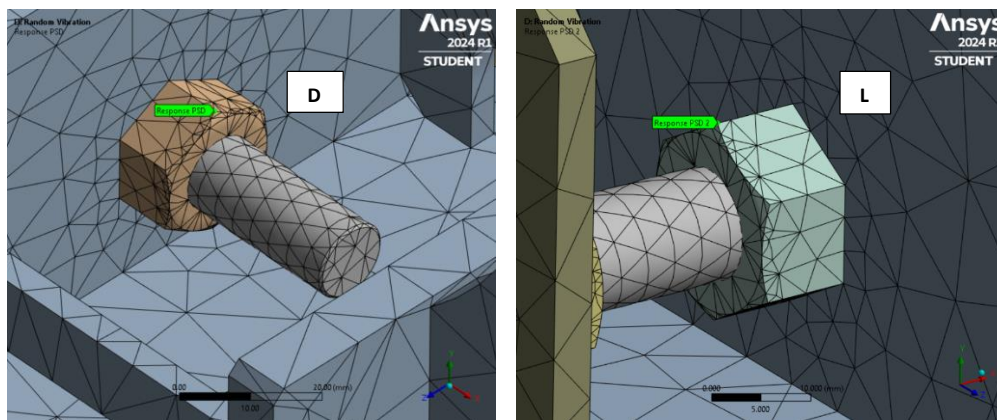
Figure 1. Vibration sampling points on the inner (D) and outer (L) bracket M12 nuts
