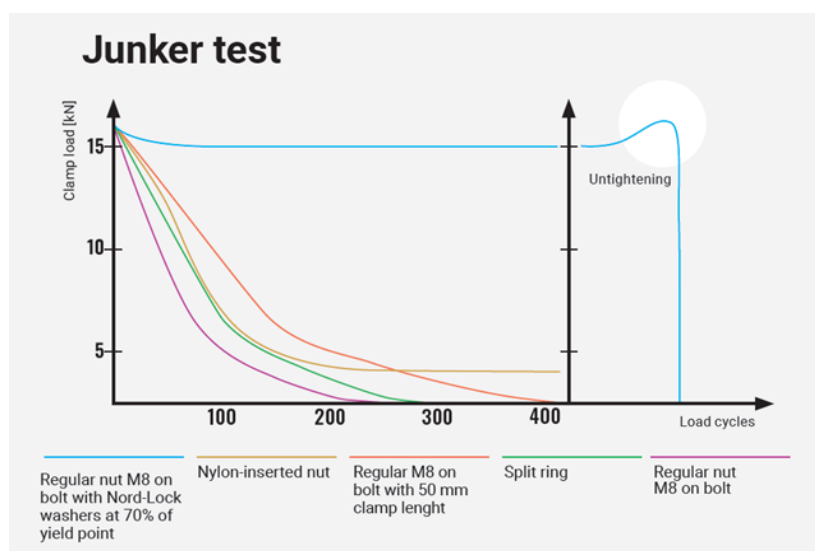
Figure 4. Graph from the Junker vibration test
