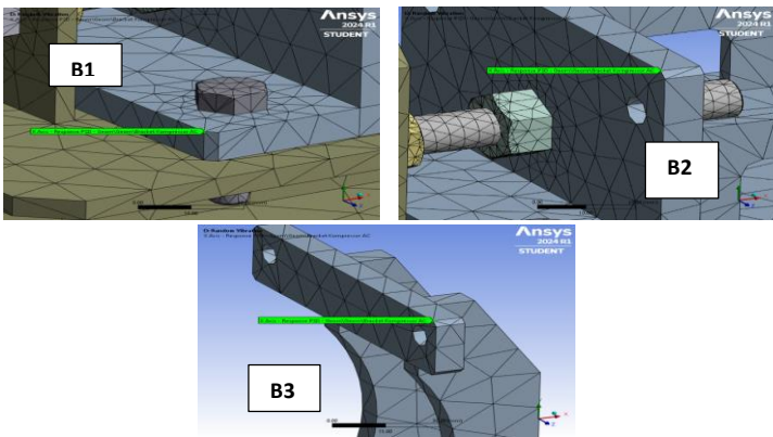
Source: Researcher, 2024 Figure 2. Vibration sampling points on the compressor
